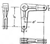
Figs. 698-700. Bell Crank for Damper Rigging.
